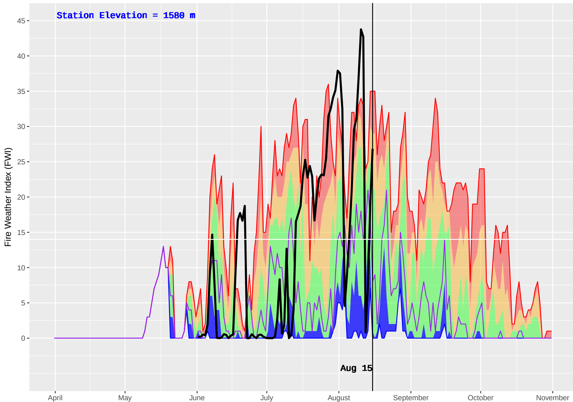
RORY CREEK (1092) : Historical (2010–2016) and Current (2018) Daily Fire Weather Index (FWI)
